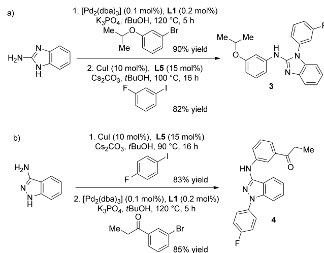
Scheme 2. Selective syntheses of diarylaminoazoles.
