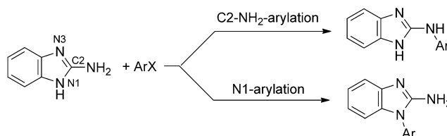
Scheme 1. Chemoselective arylation of 2-aminobenzimidazole.
